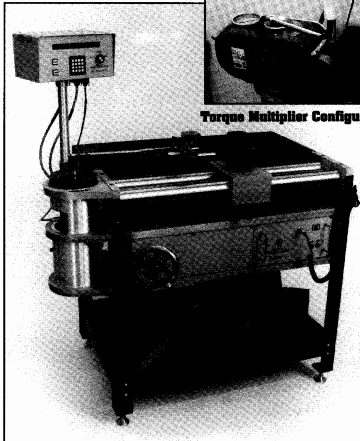
Torque Wrench Test
